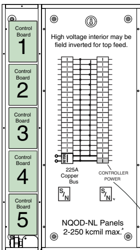
NQOD Panel 225A Copper Bus
