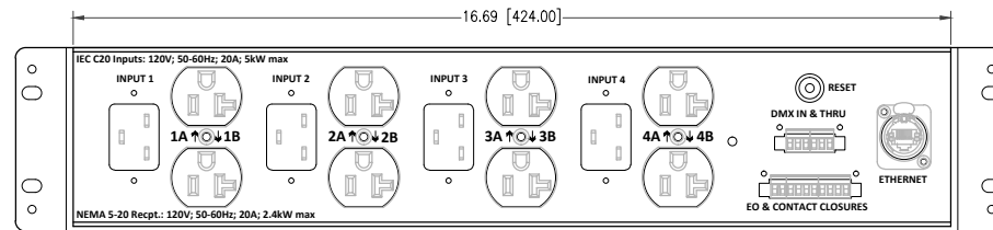
REAR VIEW
